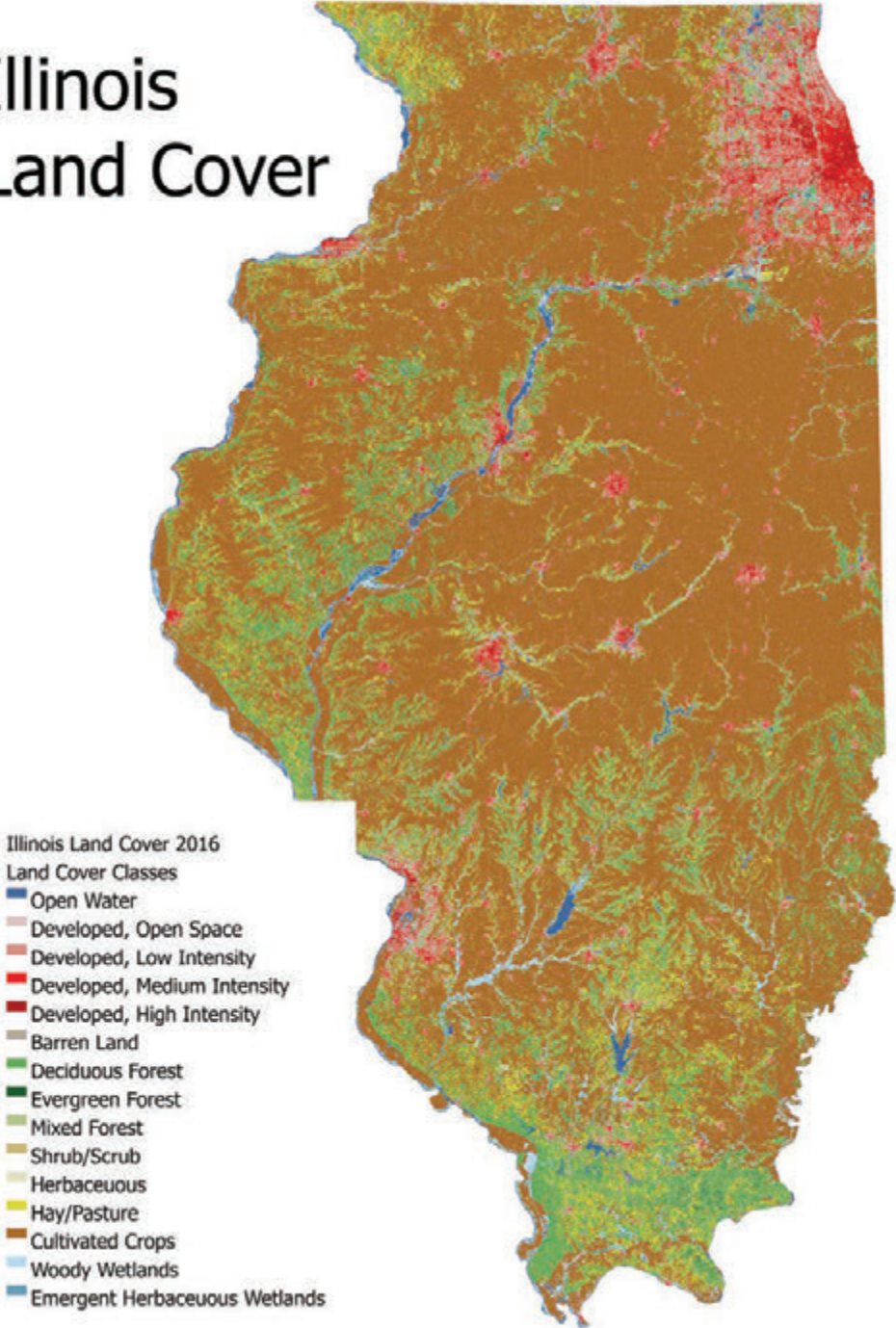
Figure 2.1. Illinois Land Cover 2016
