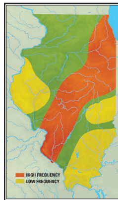
Areas of relative frequencies of tornadoes in Illinois
