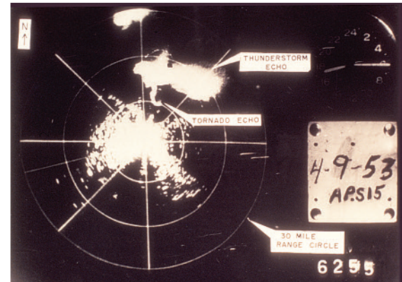
The State Water Survey's early research radar was the first in the nation to detect a tornado in April 1953. This scope photo shows the thunderstorm echo and its hook, the tornado funnel, north of the radar site near Champaign.
